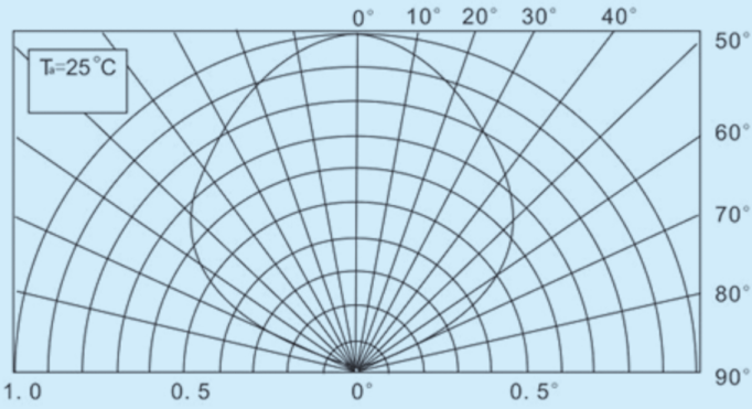
Candle Power Distribution Curve
